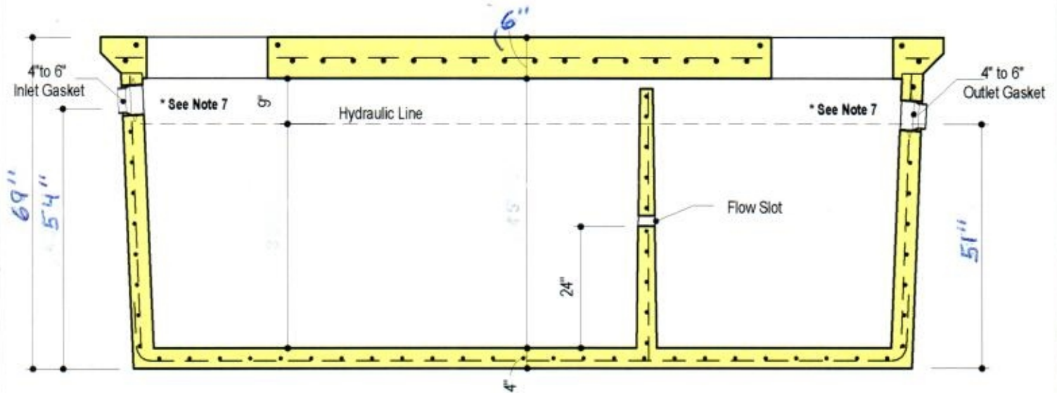
SECTION VIEW
