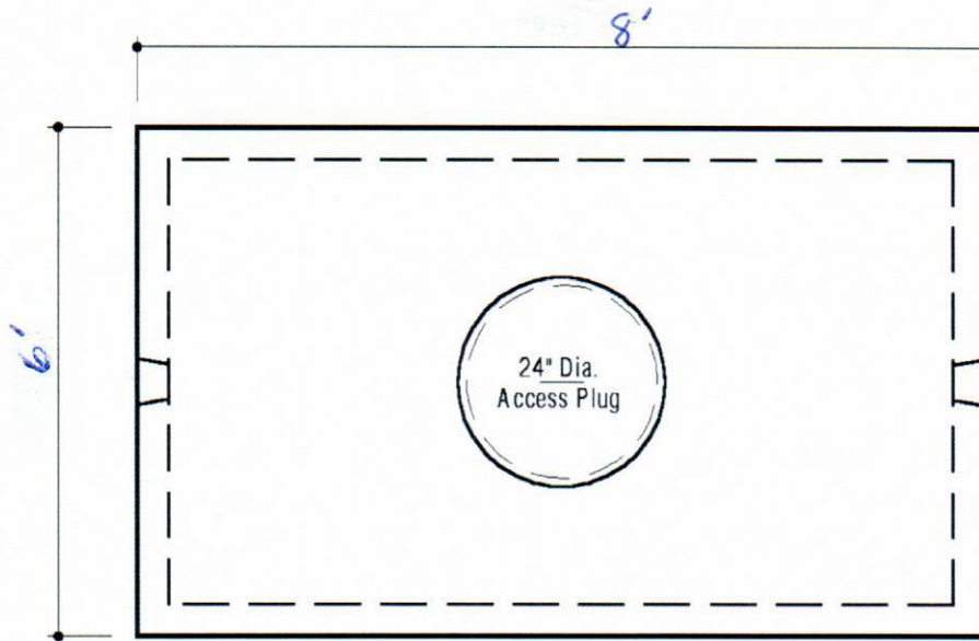
PLAN VIEW
